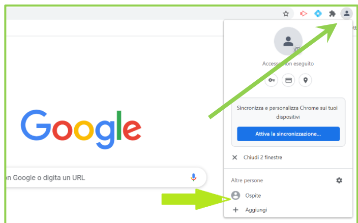
GOOGLE CHROME
